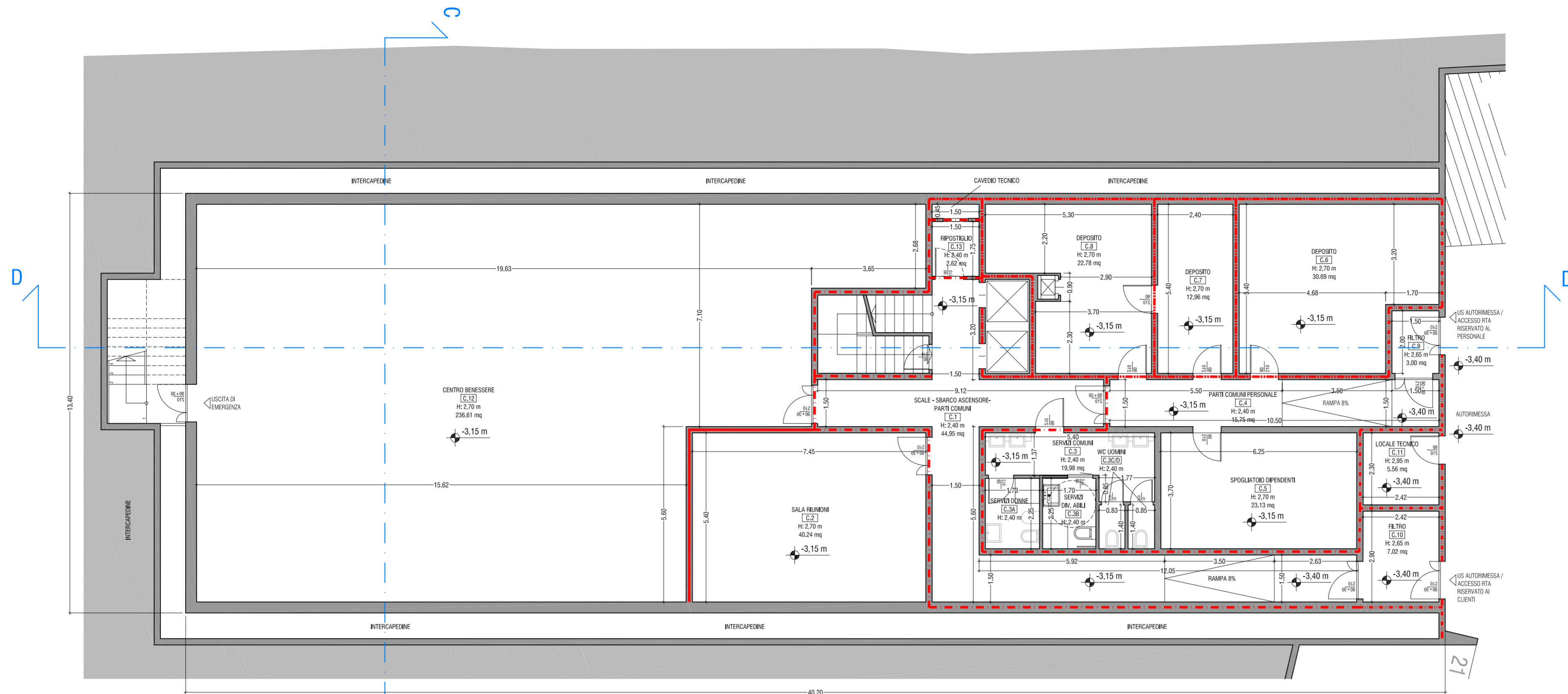
PIANO INTERRATO
