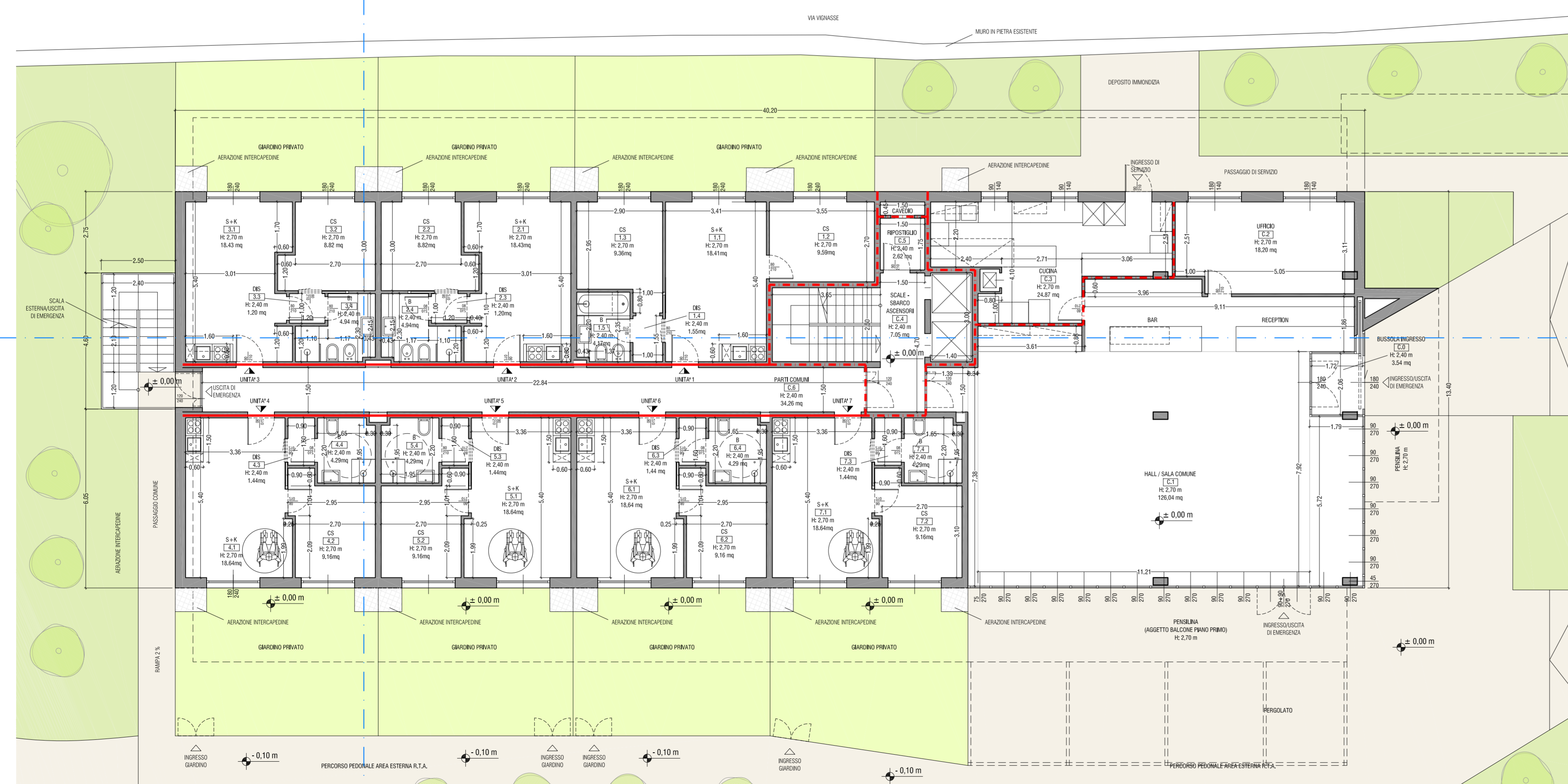
PIANO TERRA
